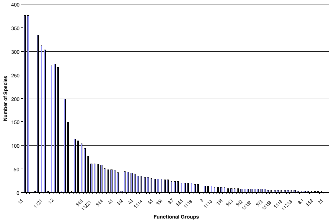
Figure 3. Number of species in each detailed functional group.
