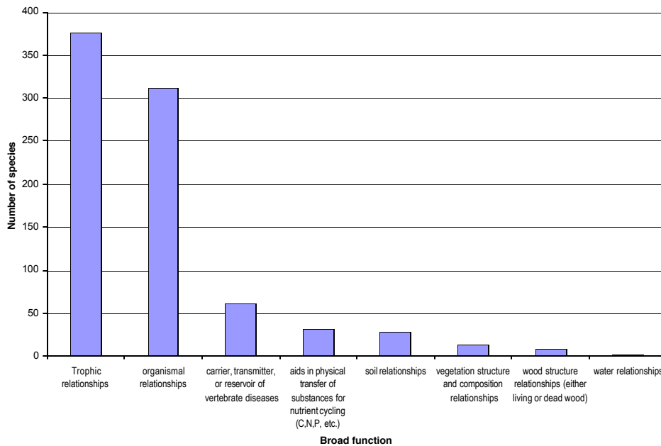
Figure 2. Number of species in each broad functional group.
